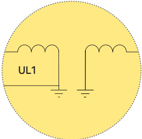
Should the voltage transformer connection be phase to phase the voltage measuring mode is selected 1LL
