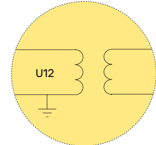
When the voltage transformer is connected to transform the phase to ground voltage, the voltage measuring mode shall be 1LN
