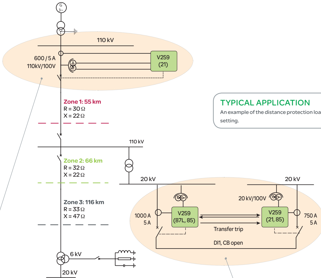
Impedance diagram
