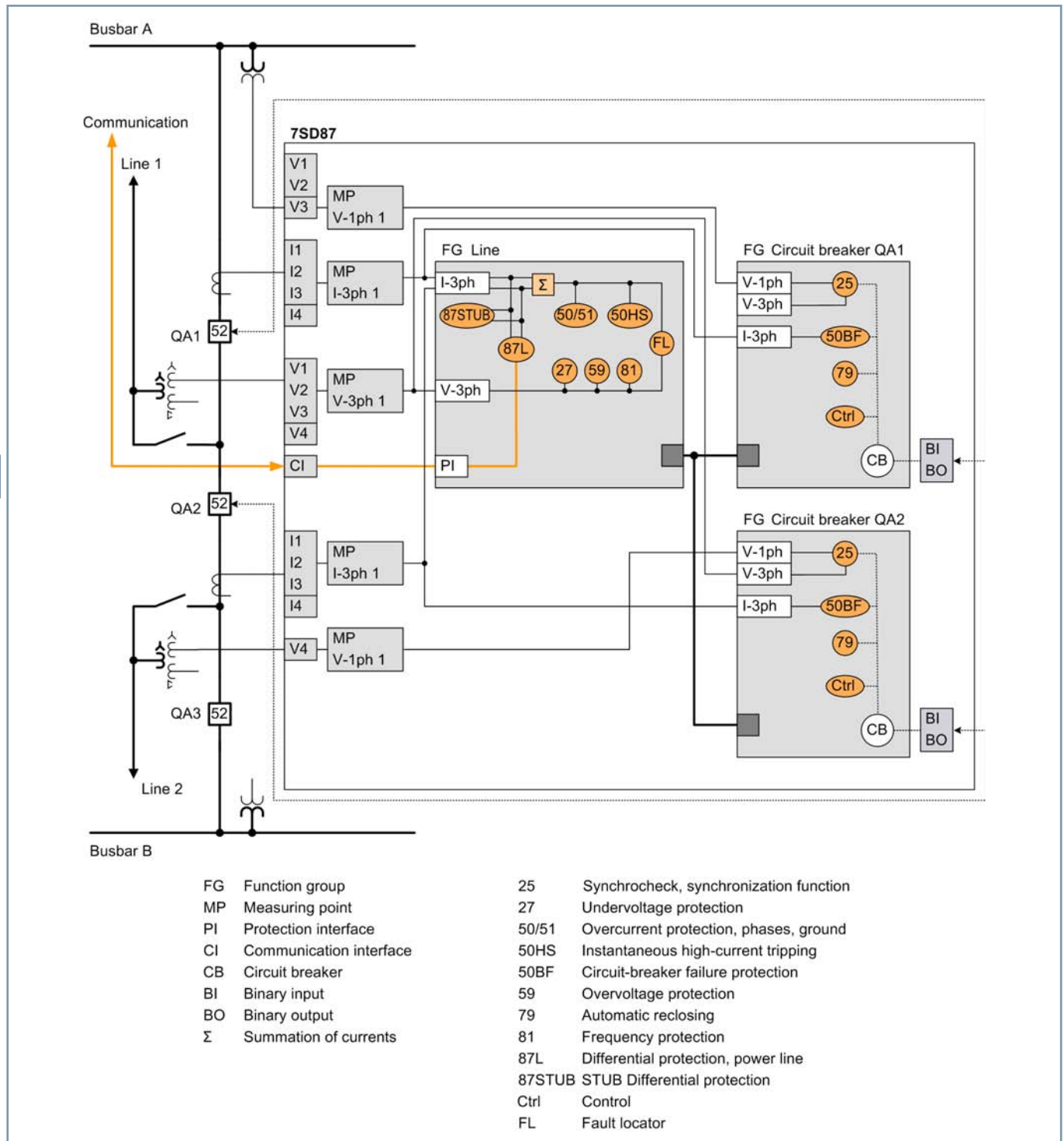
Figure 2.7/8 Application example: Line differential protection for overhead line with breaker-and-a-half scheme
